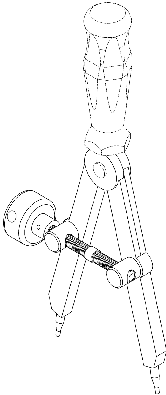
立體圖1
