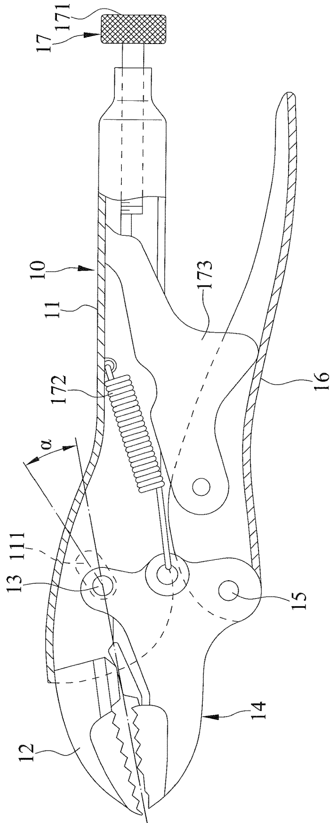
FIG. 1 PRIOR ART
